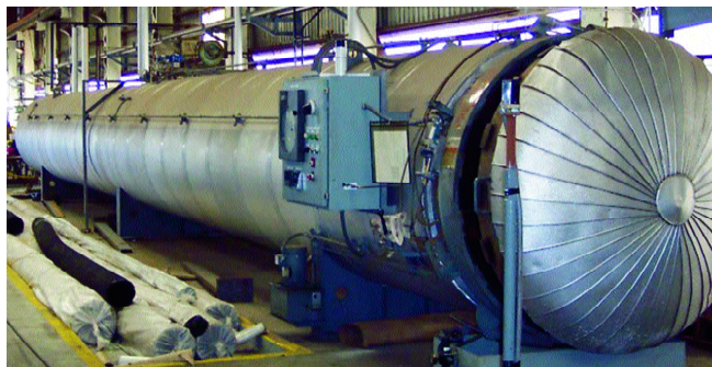
Autoclave for steam curing large diameter hoses
