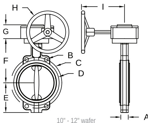
10" - 12" wafer
