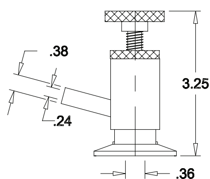
CLAMP STYLE
