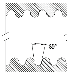
female thread
