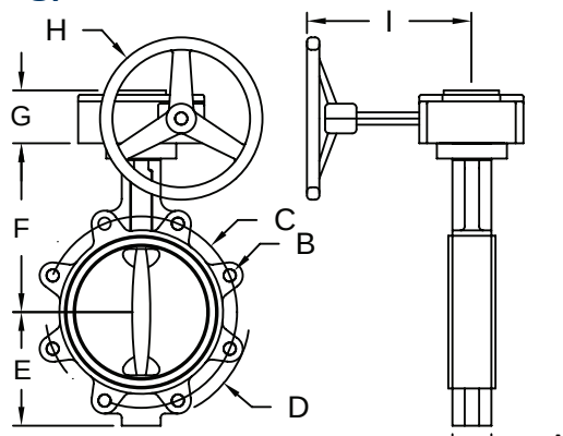
10" - 12" wafer
