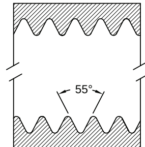
female thread
