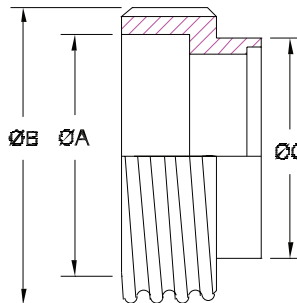
Weld Male
