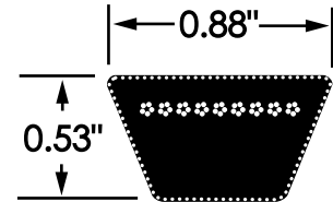
87 C SECTION
