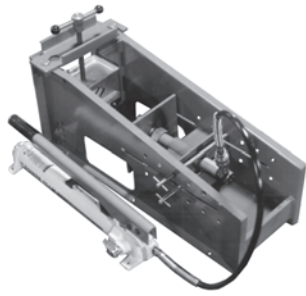
coupling inserter
