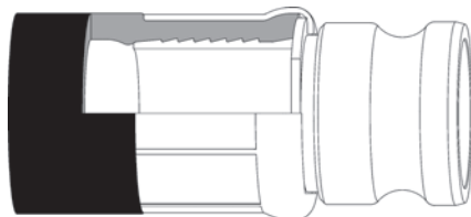
Crimped Assembly
