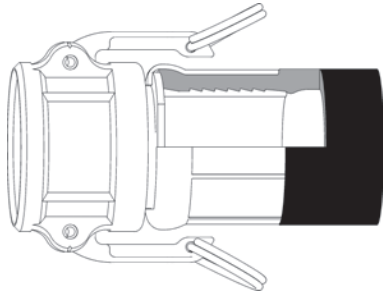
Crimped Assembly
