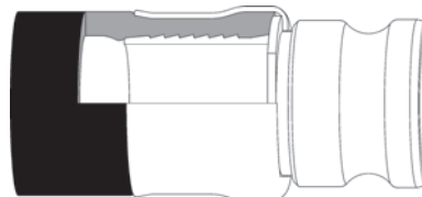
Swaged Assembly
